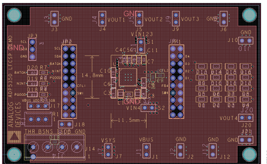
Figure 19. Third Layer, Recommended Layout for the ADP5350CP-EVALZ Evaluation Board
