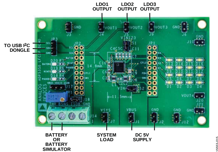
Figure 15. ADP5350CP-EVALZ LFCSP Board Connection Diagram
