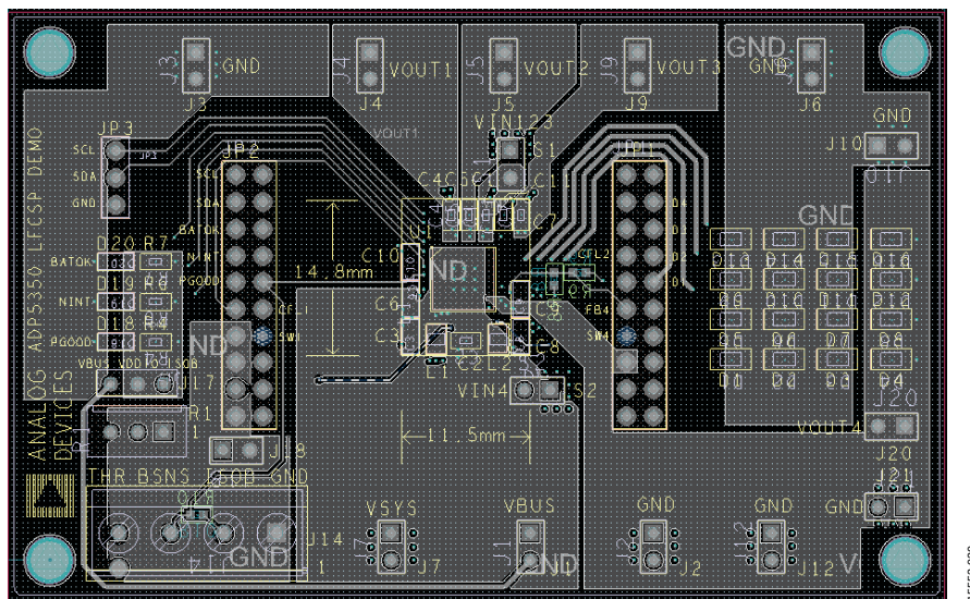
Figure 20. Bottom Layer, Recommended Layout for the ADP5350CP-EVALZ Evaluation Board
