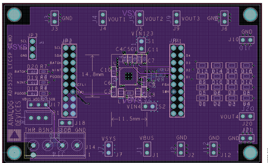
Figure 18. Second Layer, Recommended Layout for the ADP5350CP-EVALZ Evaluation Board
